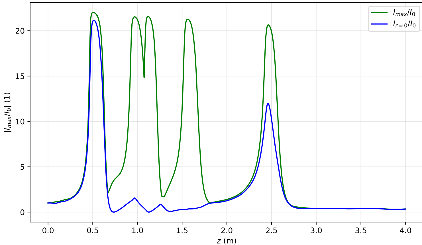
I_{max}(x=0, y=0, z)/I_0 , P_{in}=5.0P_{cr} , noisy input, artificial time
